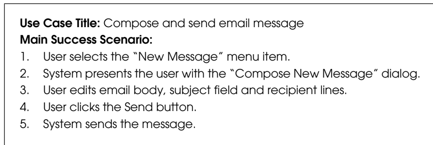
Figure 12.2 A use case to compose and send an email message.
